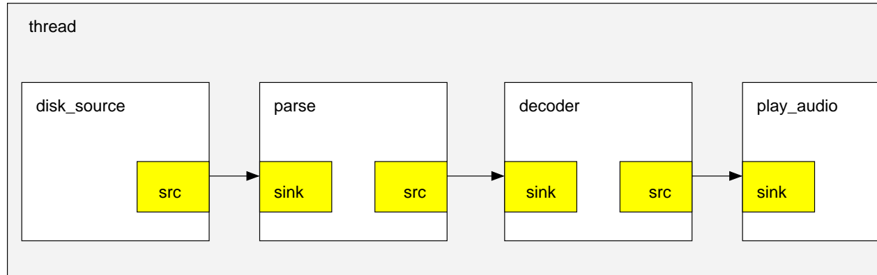
Figure 21-1. A thread
