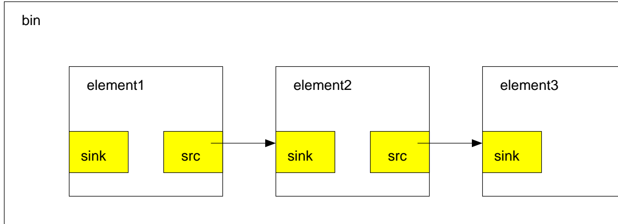
Figure 16-1. Visualisation of a GstBin 2 element without ghost pads
