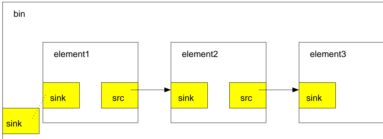
Figure 16-2. Visualisation of a GstBin 3 element with a ghost pad
